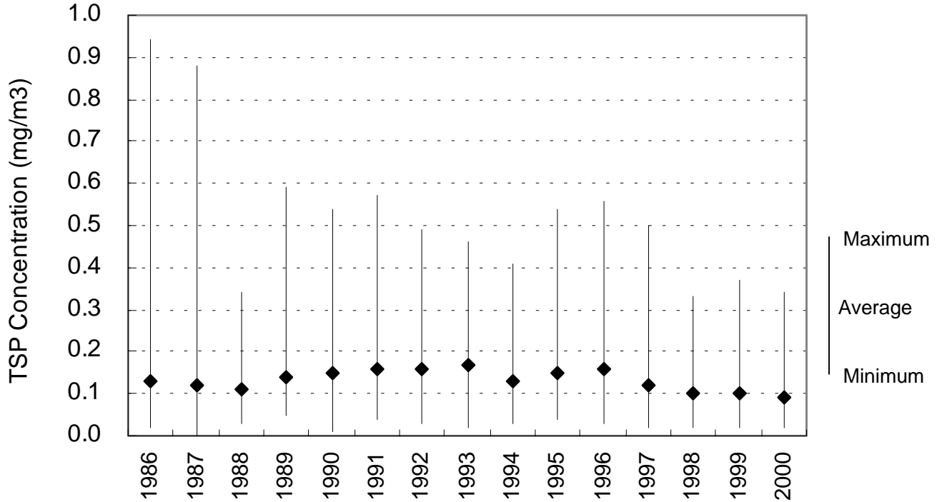
AMBIENT AIR PARTICULATE (TSP) LEVEL 1986-2000 24-Hour Average Concentration Standard = 0.33mg/m 3
