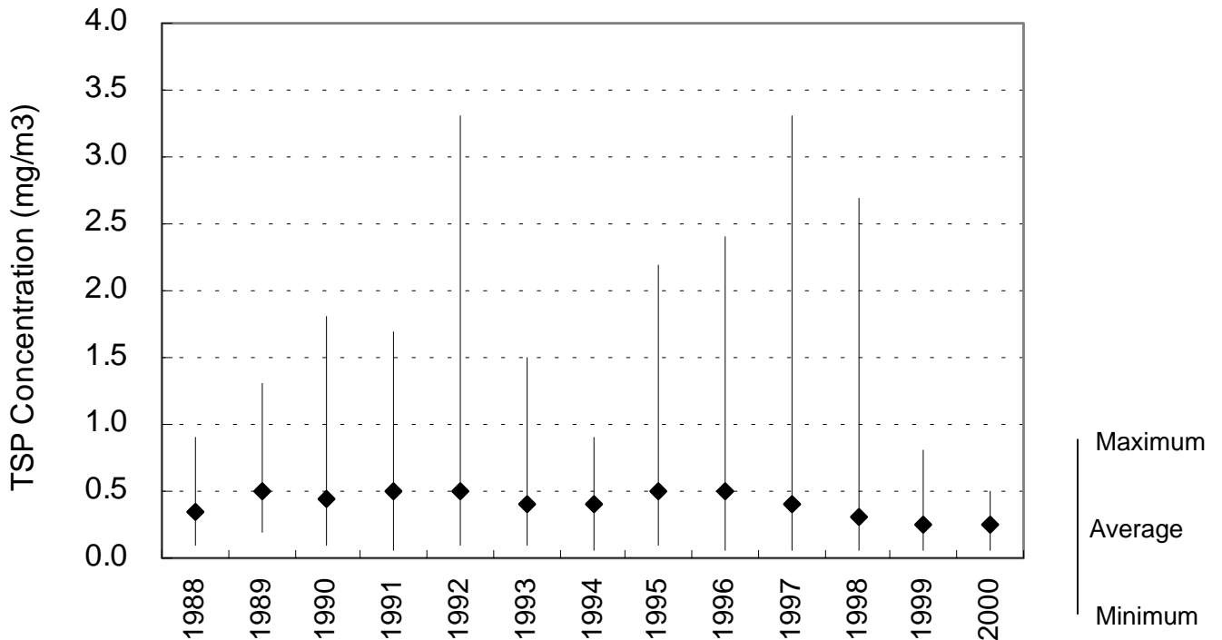
ROADSIDE AIR PARTICULATE (TSP) LEVEL 1998-2000 24-Hour Average Concentration Standard = 0.33mg/m 3
